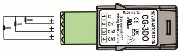
Figure 2 – Electrical connections
